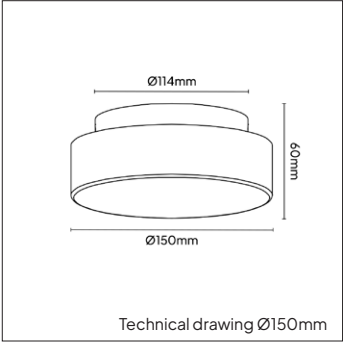
Technical drawing Ø150mm
