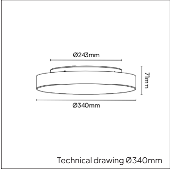
Technical drawing Ø340mm
