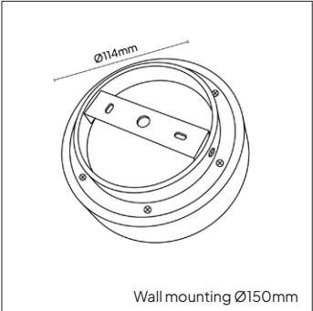
Wall mounting Ø150mm
