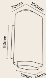
TECHNICAL DRAWING
