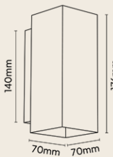
TECHNICAL DRAWING
