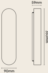
TECHNICAL DRAWING
