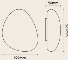
TECHNICAL DRAWING
