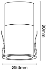
TECHNICAL DRAWING
