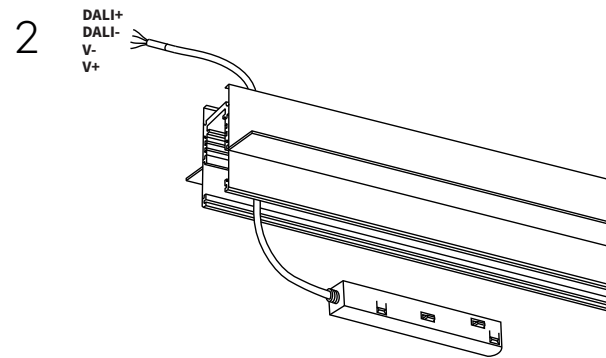
Connection schedule for Magnet XS Track Power Feed. DALI line is not used.
