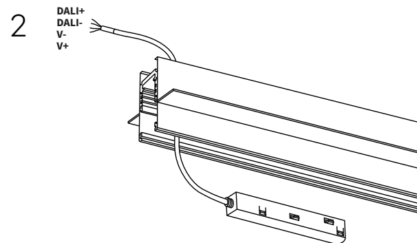
Connection schedule for Magnet XS Track Power Feed.
